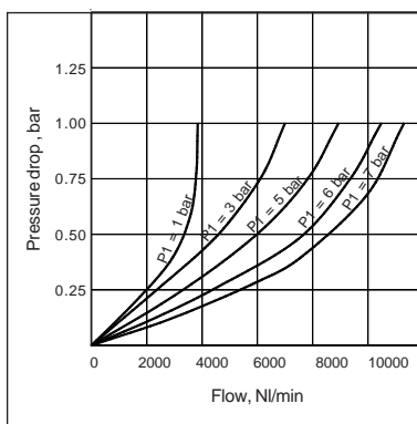
3/4" LUBRICATOR
